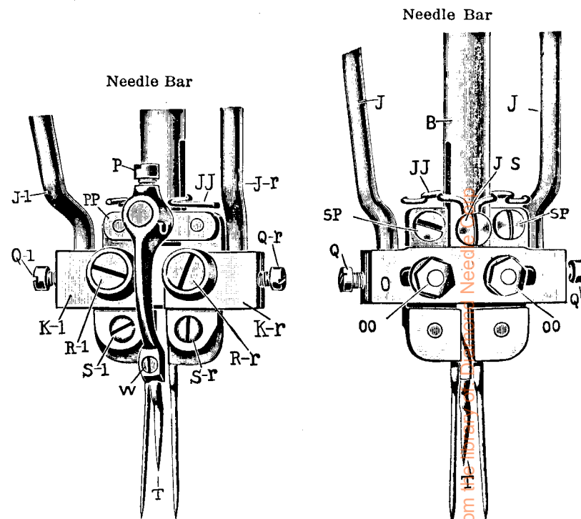
Fig. 16 Front view
